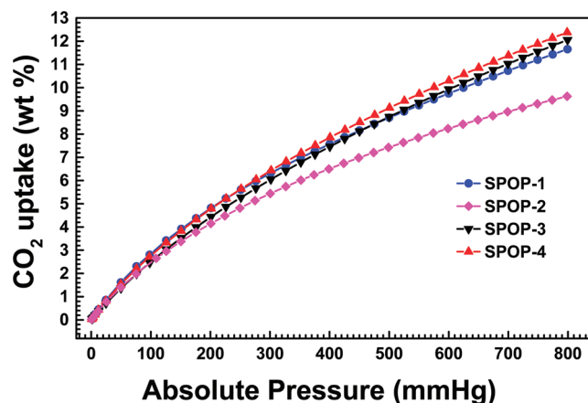
Figure 5. Gravimetric CO 2 adsorption isotherms for SPOPs at 273 K.
